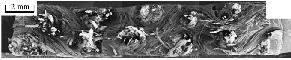
Figure 6. Fracture photographs of compact tension specimens.
