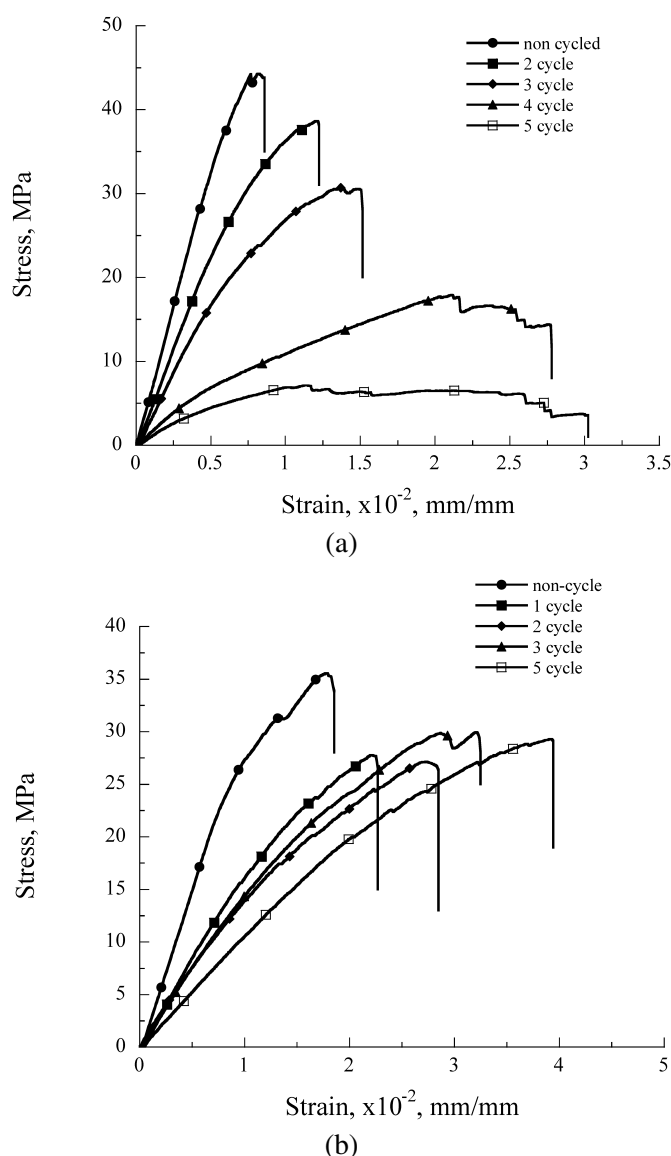
Figure 4. Stress and strain behaviors according to various cyclic times. (a) For sisal epoxy composites; (b) For sisal vinyl-ester composites.
